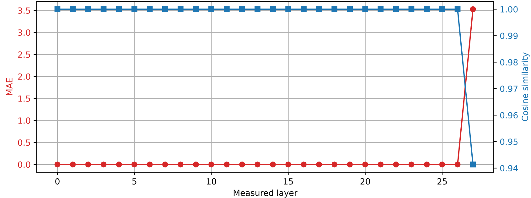
Qwen2.5-7B-Instruct | Prompt 3 Spared layer 26 | Hybrid vs quantized
