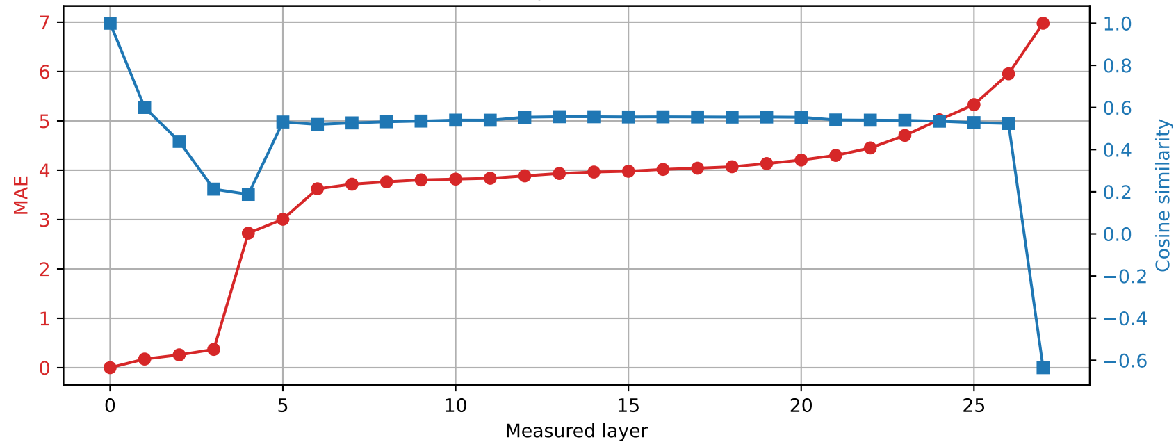
Qwen2.5-7B-Instruct | Prompt 3 Spared layer 26 | Hybrid vs unquantized
