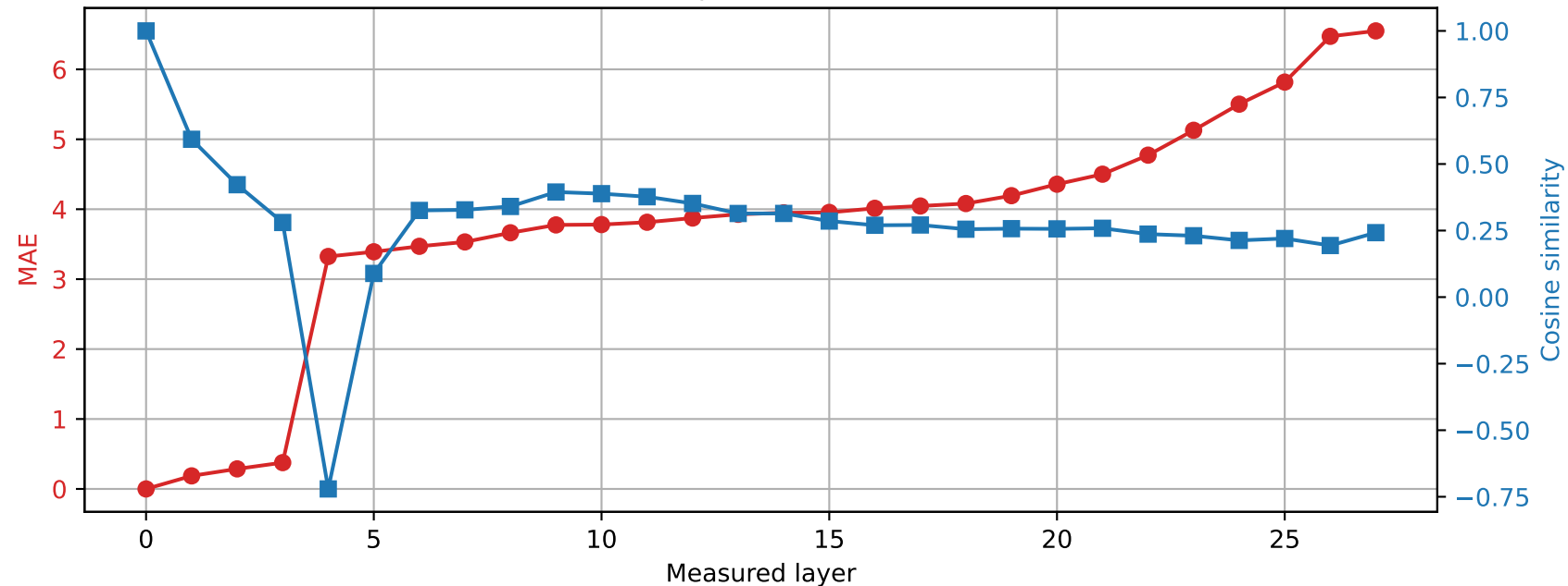
Qwen2.5-7B-Instruct | Prompt 4 Spared layer 3 | Hybrid vs unquantized
