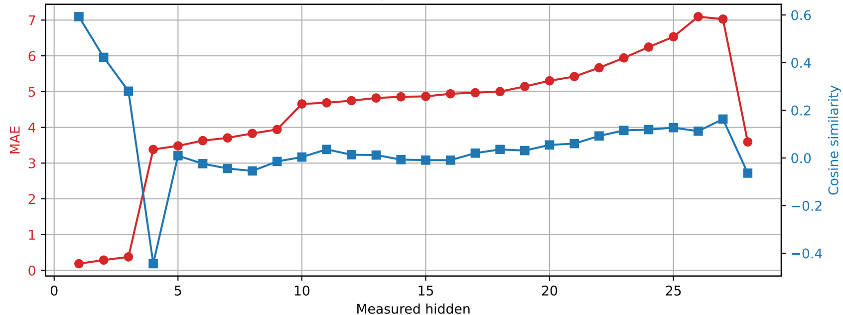
Qwen2.5-7B-Instruct | Prompt 4 Spared layer 9 | Unquantized vs hybrid
