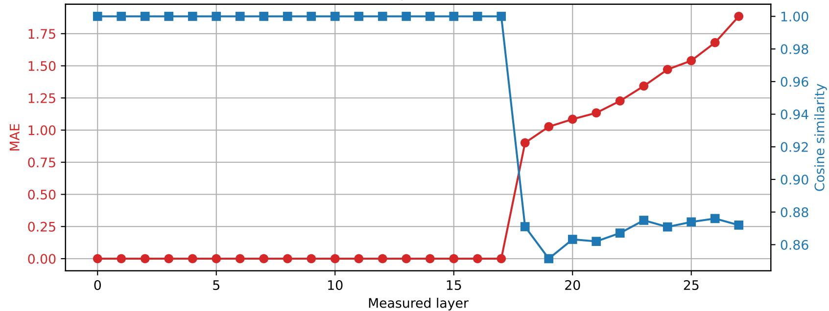
Qwen2.5-7B-Instruct | Prompt 4 Spared layer 17 | Hybrid vs quantized
