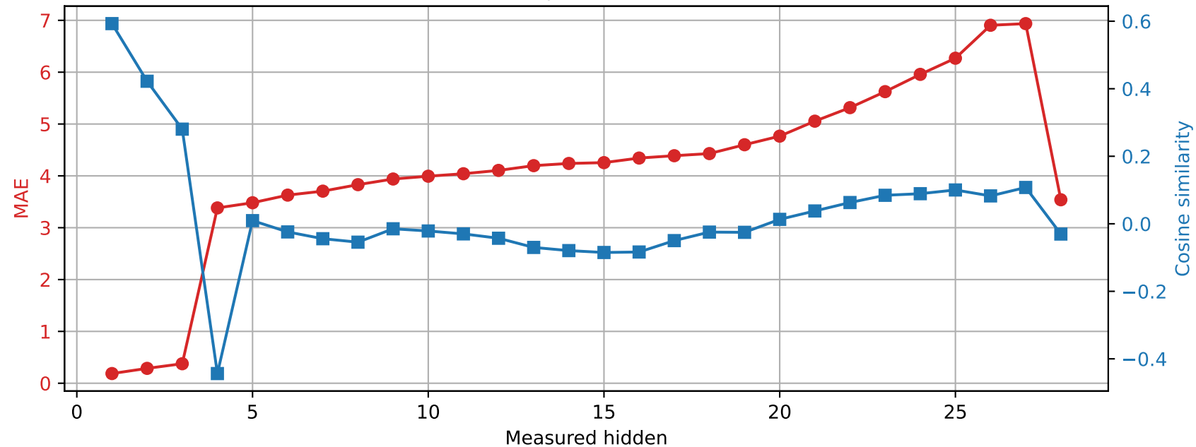
Qwen2.5-7B-Instruct | Prompt 4 Spared layer 20 | Unquantized vs hybrid
