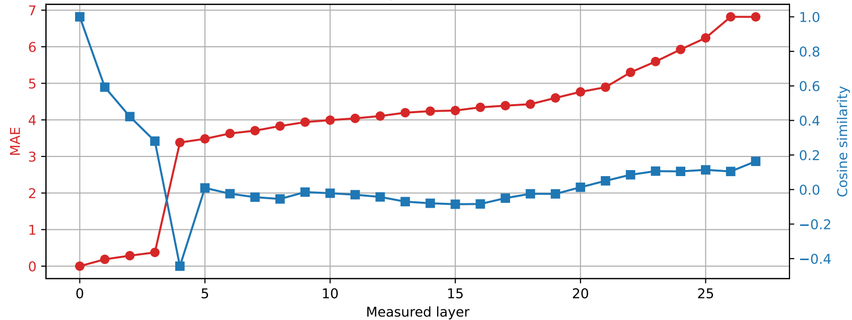
Qwen2.5-7B-Instruct | Prompt 4 Spared layer 21 | Hybrid vs unquantized
