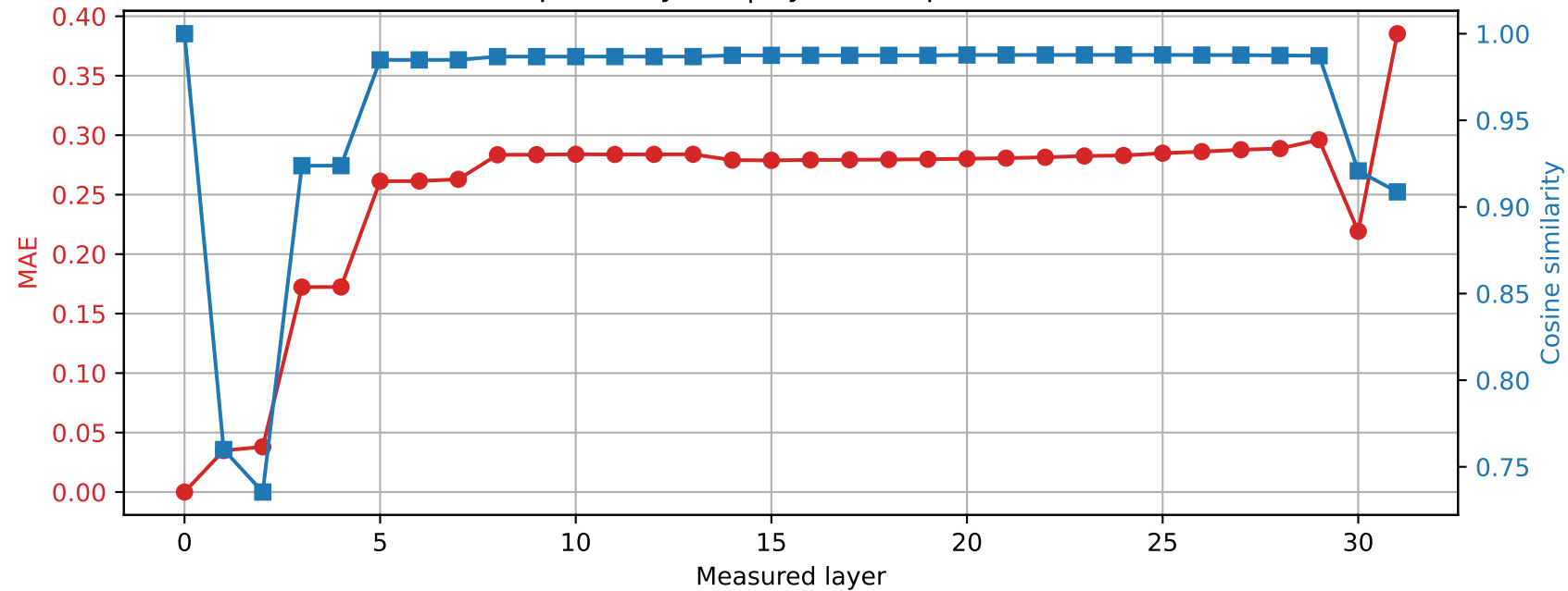
Phi-3-mini-4k-instruct | Prompt 0 Spared layer 0 | Hybrid vs quantized
