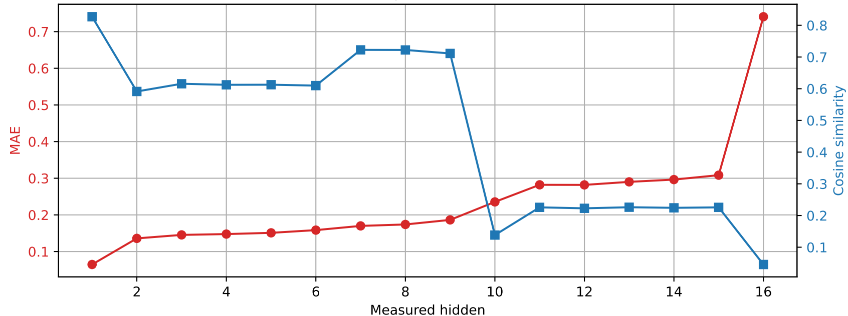
OLMo-1B-hf | Prompt 0 Spared layer 3 | Unquantized vs hybrid
