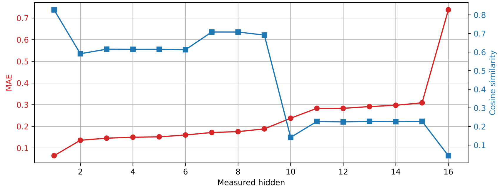
OLMo-1B-hf | Prompt 0 Spared layer 4 | Unquantized vs hybrid
