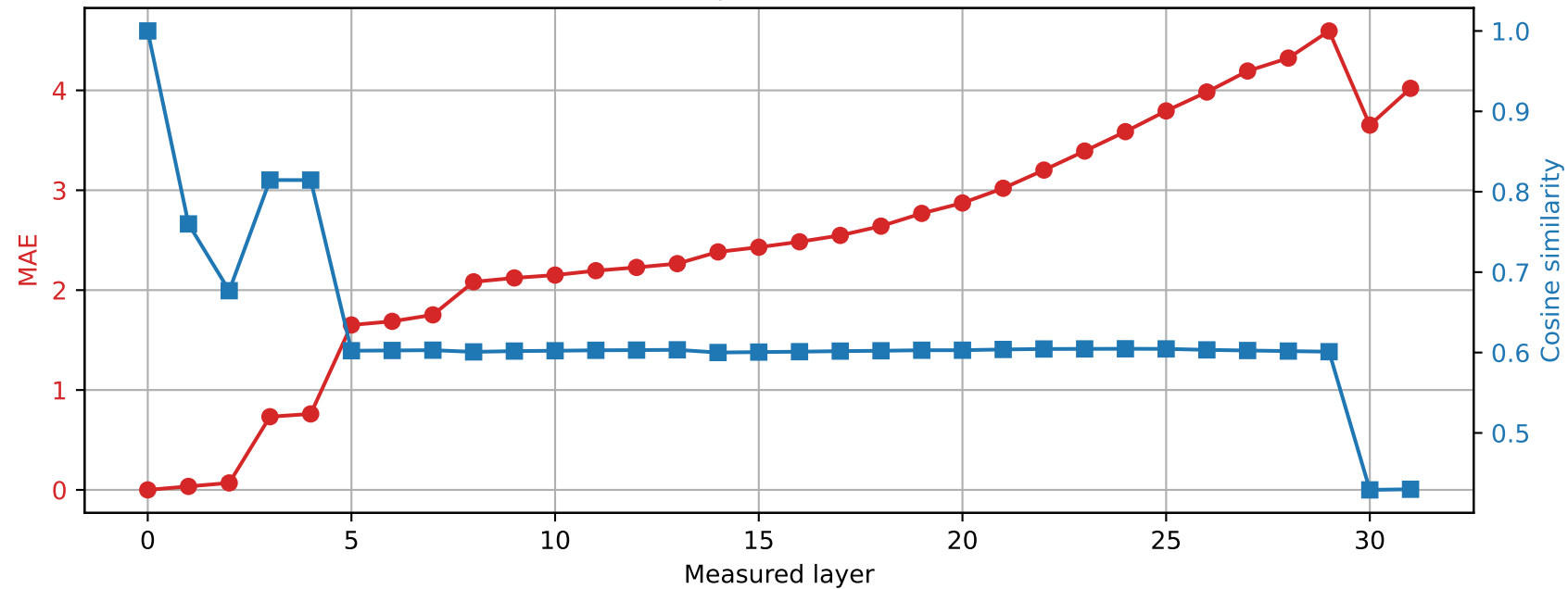
Phi-3-mini-4k-instruct | Prompt 0 Spared layer 7 | Hybrid vs unquantized
