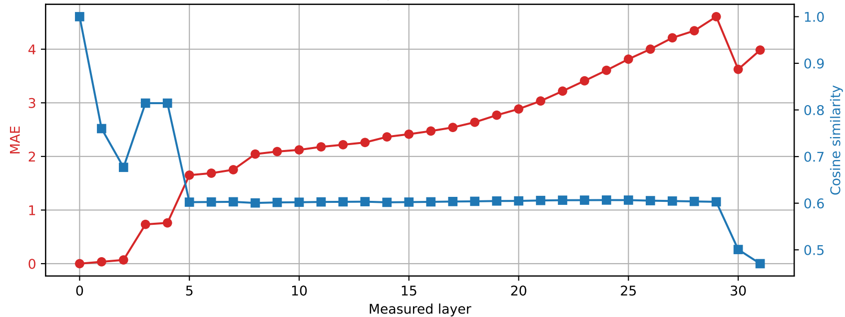
Phi-3-mini-4k-instruct | Prompt 0 Spared layer 8 | Hybrid vs unquantized
