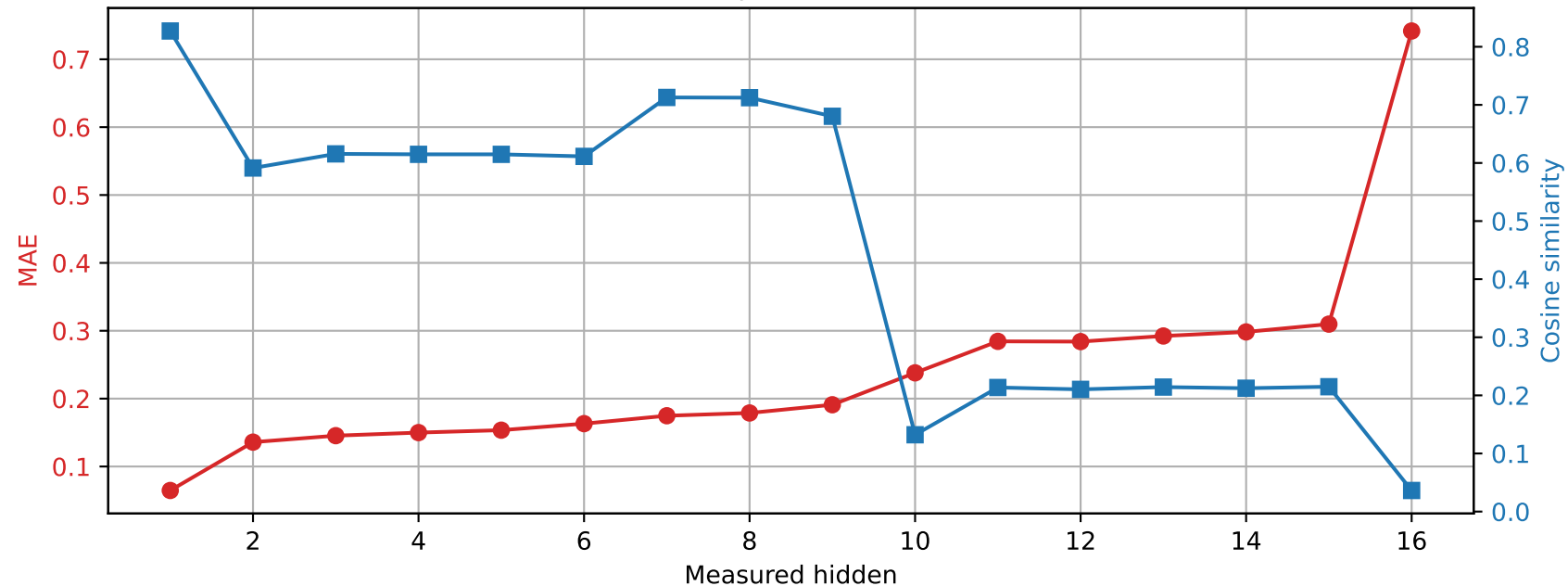
OLMo-1B-hf | Prompt 0 Spared layer 14 | Unquantized vs hybrid
