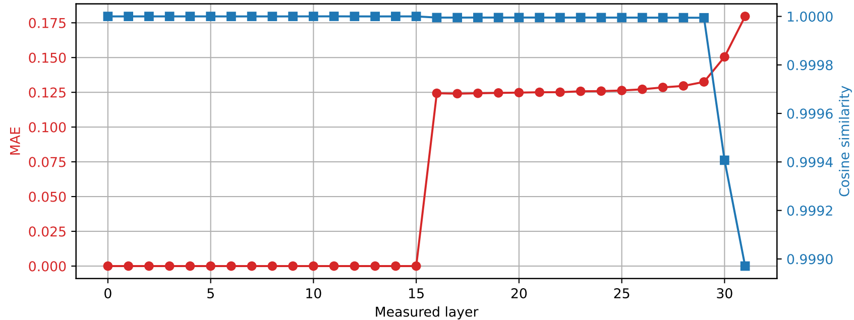
Phi-3-mini-4k-instruct | Prompt 0 Spared layer 15 | Hybrid vs quantized
