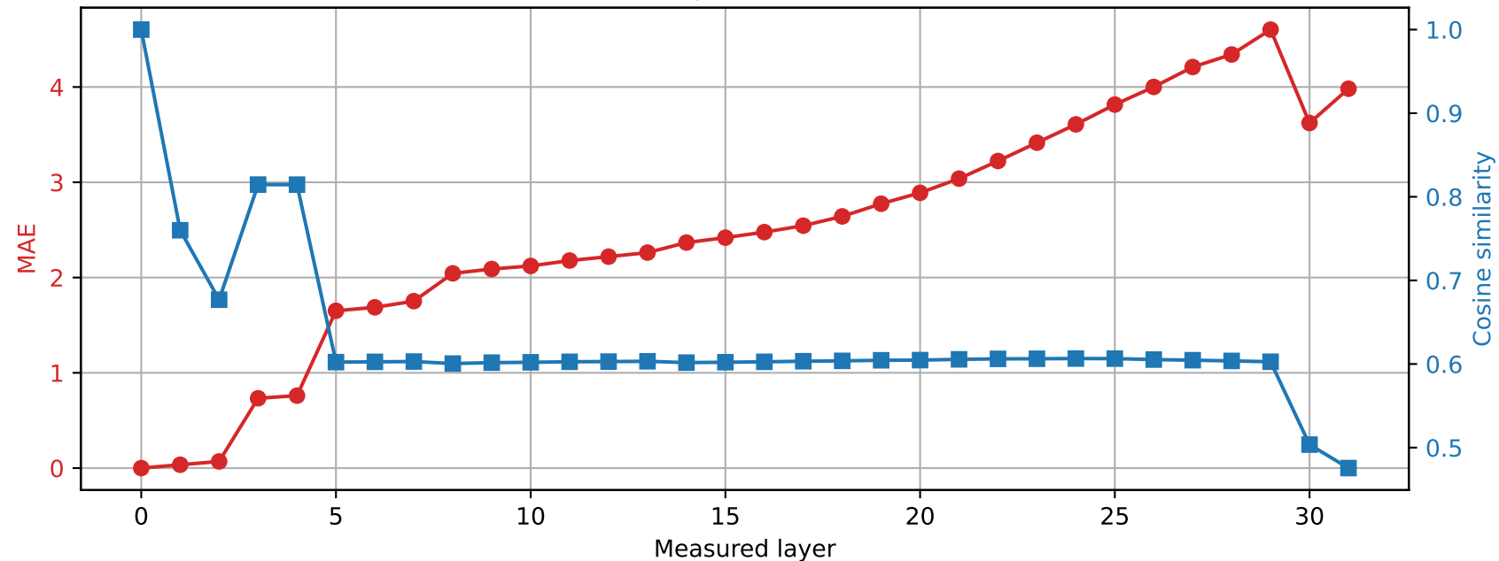
Phi-3-mini-4k-instruct | Prompt 0 Spared layer 23 | Hybrid vs unquantized
