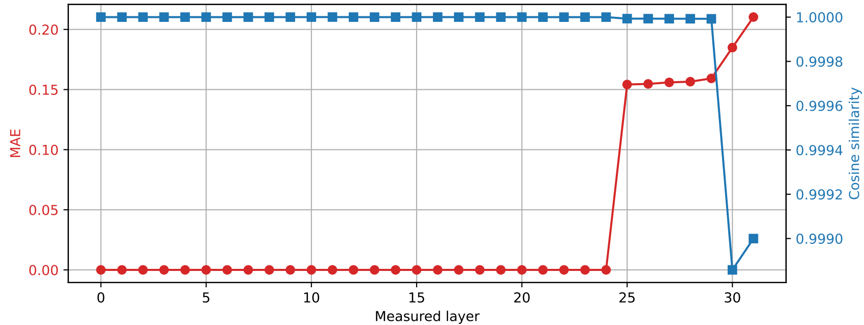
Phi-3-mini-4k-instruct | Prompt 0 Spared layer 24 | Hybrid vs quantized
