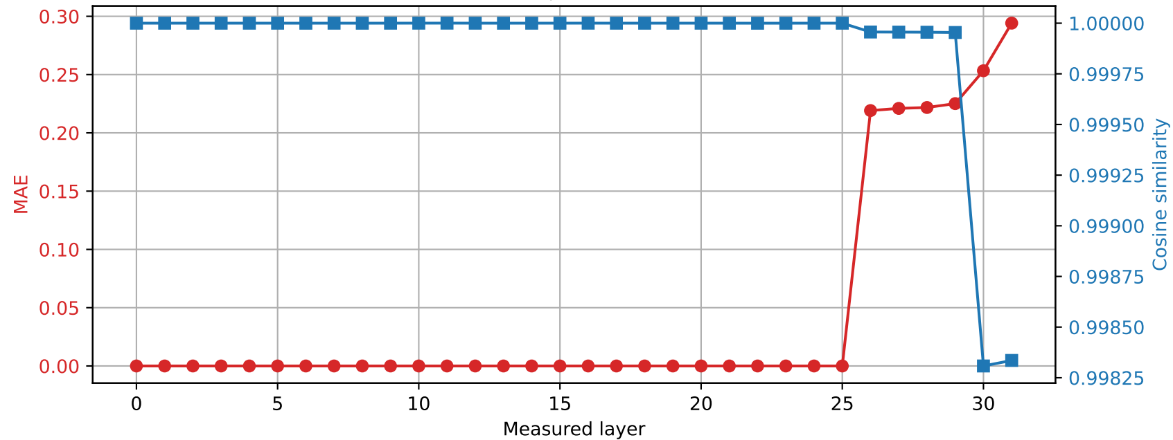
Phi-3-mini-4k-instruct | Prompt 0 Spared layer 25 | Hybrid vs quantized
