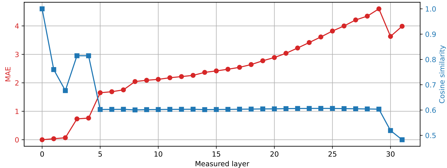
Phi-3-mini-4k-instruct | Prompt 0 Spared layer 25 | Hybrid vs unquantized
