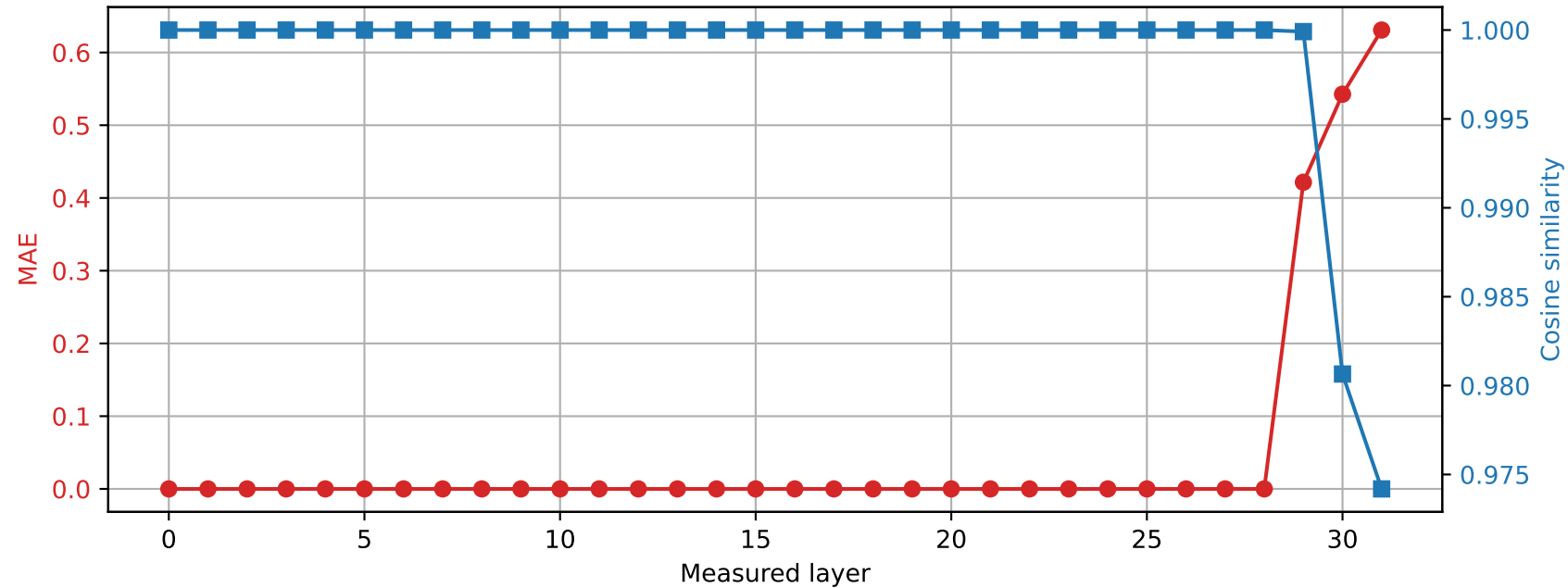
Phi-3-mini-4k-instruct | Prompt 0 Spared layer 28 | Hybrid vs quantized
