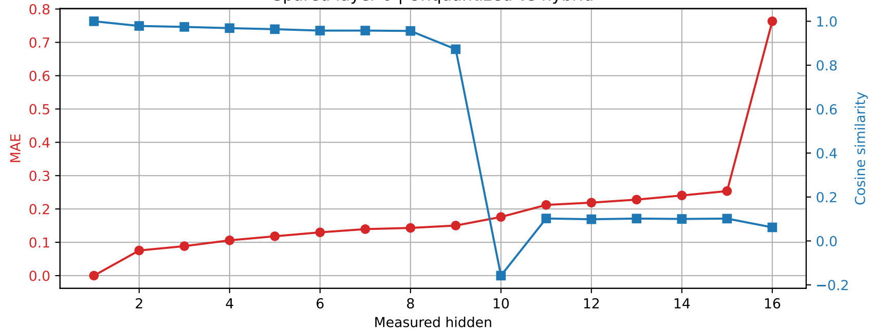
OLMo-1B-hf | Prompt 1 Spared layer 0 | Unquantized vs hybrid
