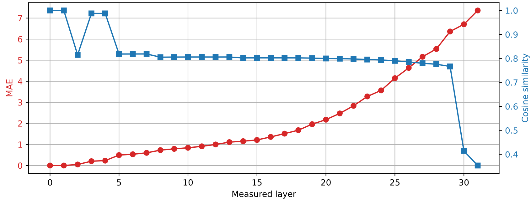
Phi-3-mini-4k-instruct | Prompt 1 Spared layer 0 | Hybrid vs unquantized
