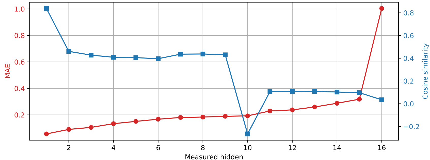
OLMo-1B-hf | Prompt 1 Spared layer 1 | Unquantized vs hybrid
