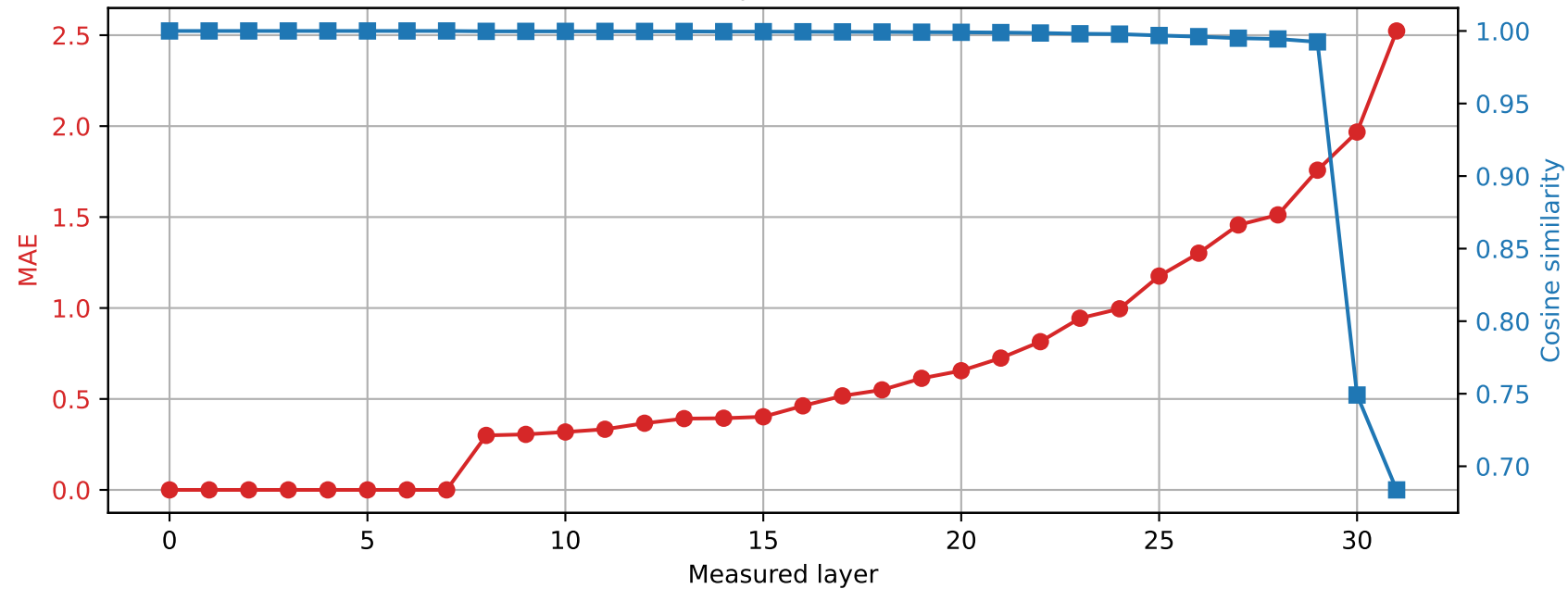
Phi-3-mini-4k-instruct | Prompt 1 Spared layer 7 | Hybrid vs quantized
