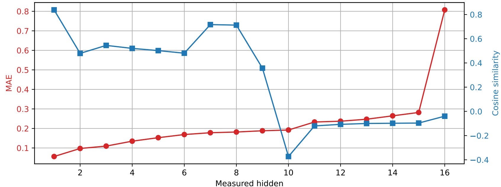
OLMo-1B-hf | Prompt 1 Spared layer 10 | Unquantized vs hybrid
