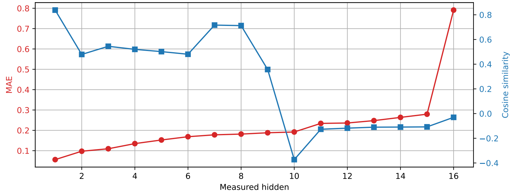
OLMo-1B-hf | Prompt 1 Spared layer 12 | Unquantized vs hybrid
