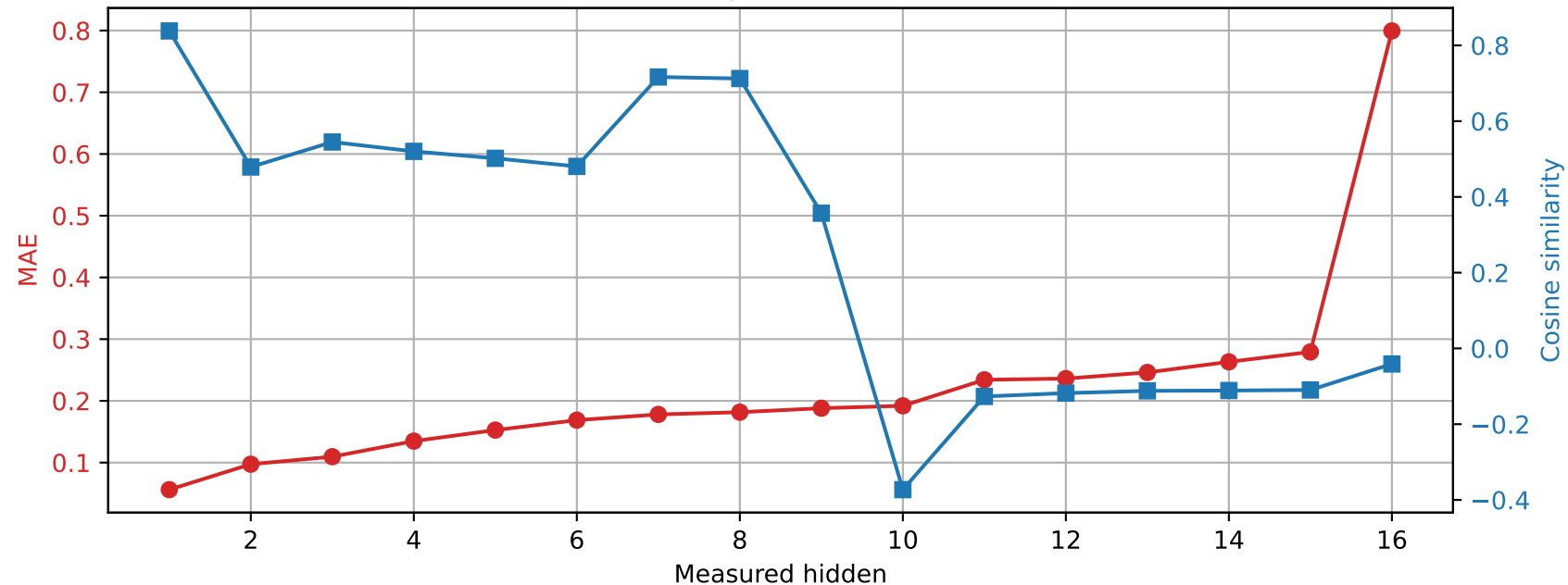
OLMo-1B-hf | Prompt 1 Spared layer 13 | Unquantized vs hybrid
