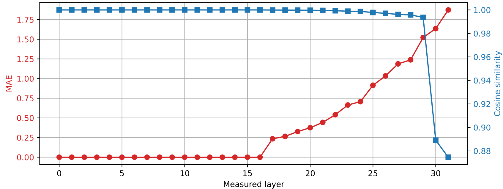
Phi-3-mini-4k-instruct | Prompt 1 Spared layer 16 | Hybrid vs quantized
