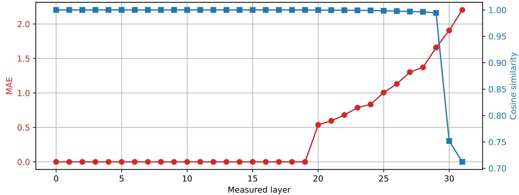
Phi-3-mini-4k-instruct | Prompt 1 Spared layer 19 | Hybrid vs quantized
