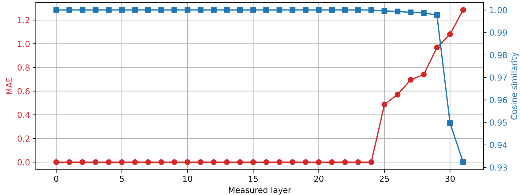
Phi-3-mini-4k-instruct | Prompt 1 Spared layer 24 | Hybrid vs quantized
