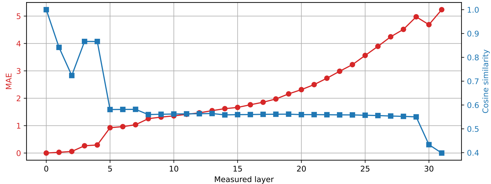
Phi-3-mini-4k-instruct | Prompt 1 Spared layer 26 | Hybrid vs unquantized
