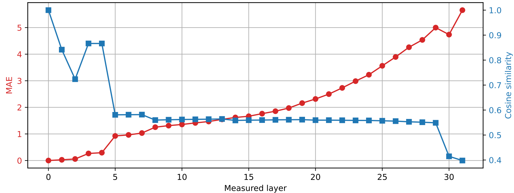
Phi-3-mini-4k-instruct | Prompt 1 Spared layer 30 | Hybrid vs unquantized
