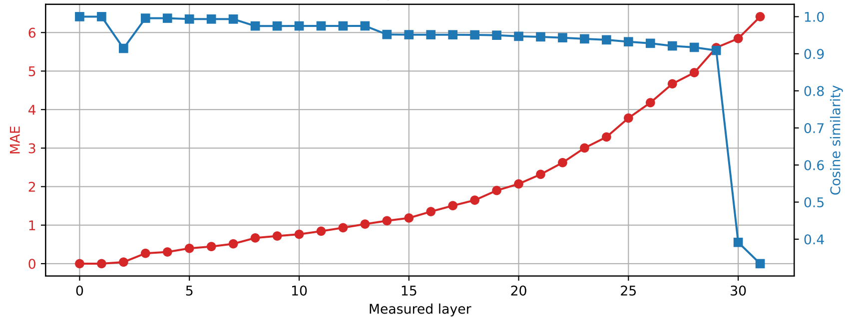
Phi-3-mini-4k-instruct | Prompt 2 Spared layer 0 | Hybrid vs unquantized
