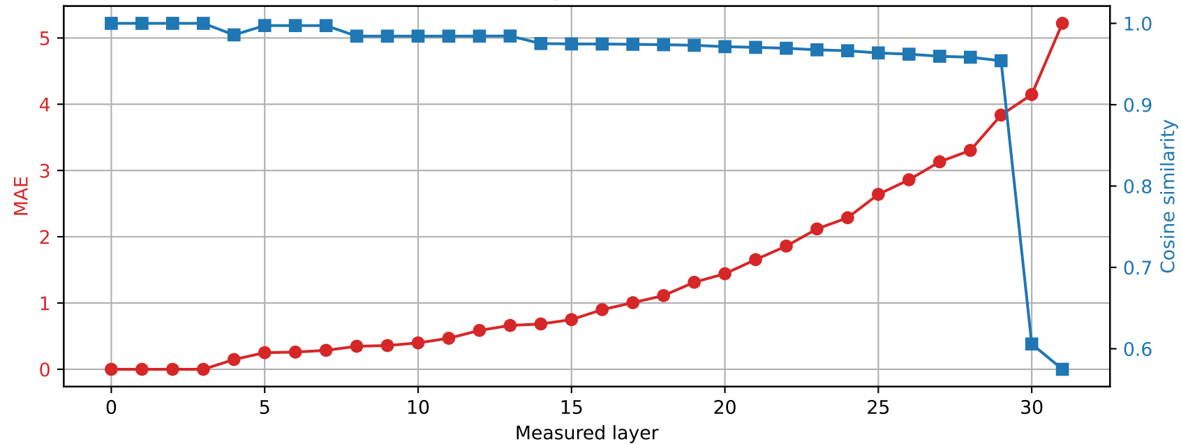
Phi-3-mini-4k-instruct | Prompt 2 Spared layer 3 | Hybrid vs quantized
