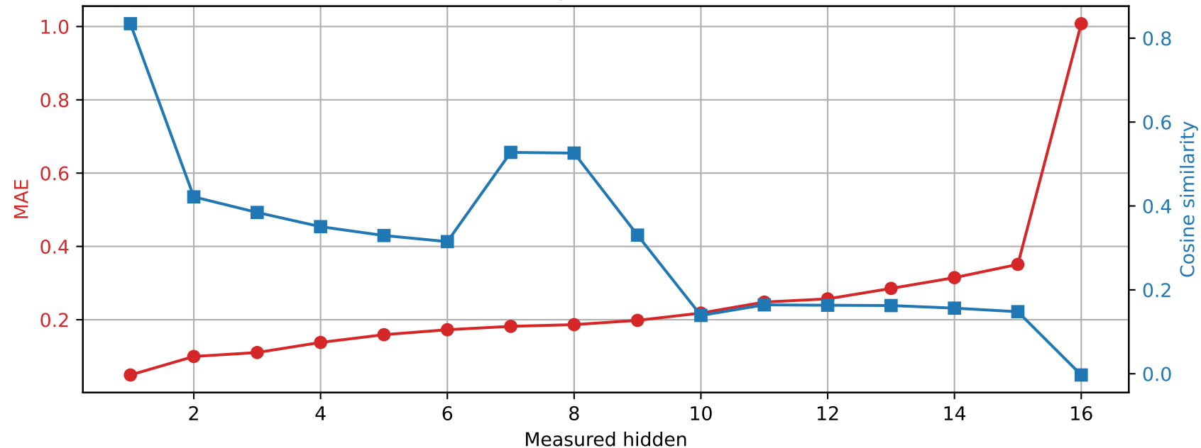
OLMo-1B-hf | Prompt 2 Spared layer 9 | Unquantized vs hybrid
