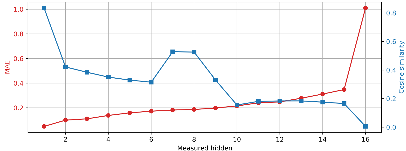
OLMo-1B-hf | Prompt 2 Spared layer 10 | Unquantized vs hybrid
