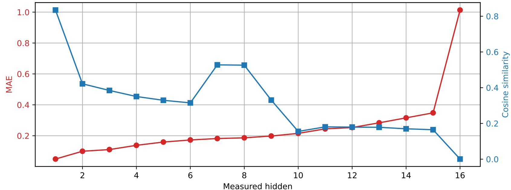
OLMo-1B-hf | Prompt 2 Spared layer 14 | Unquantized vs hybrid
