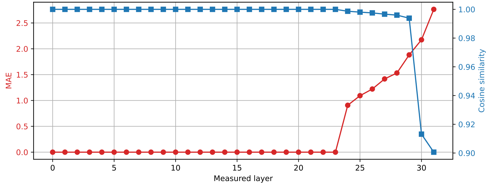
Phi-3-mini-4k-instruct | Prompt 2 Spared layer 23 | Hybrid vs quantized
