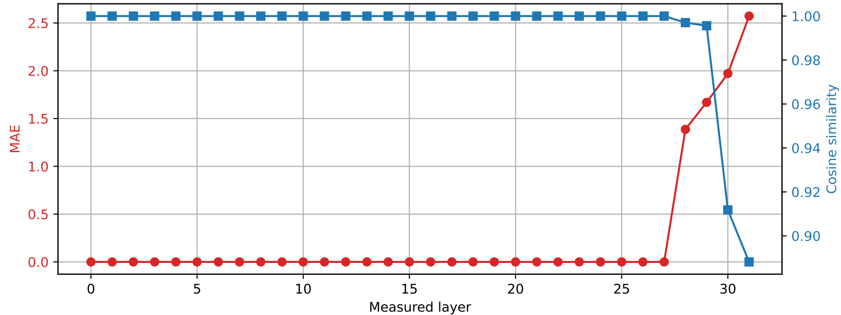
Phi-3-mini-4k-instruct | Prompt 2 Spared layer 27 | Hybrid vs quantized
