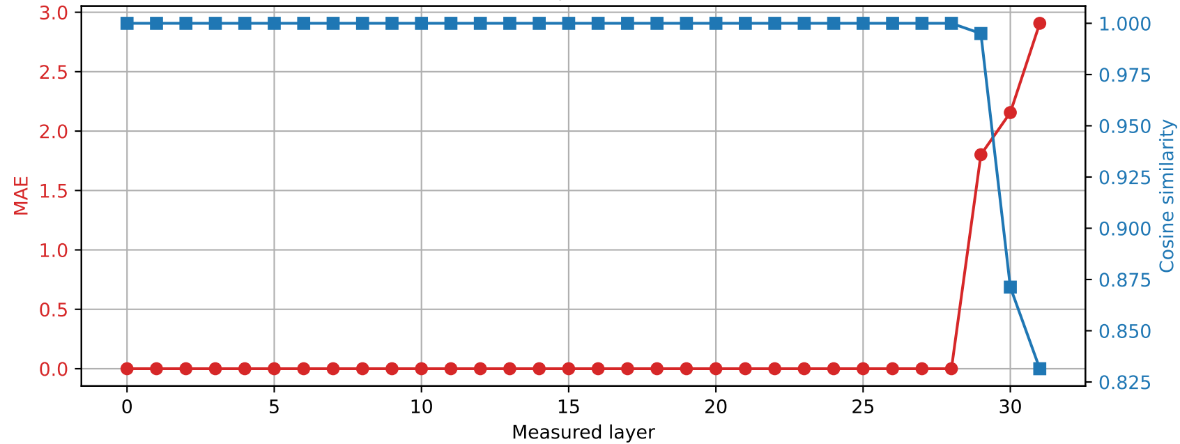
Phi-3-mini-4k-instruct | Prompt 2 Spared layer 28 | Hybrid vs quantized
