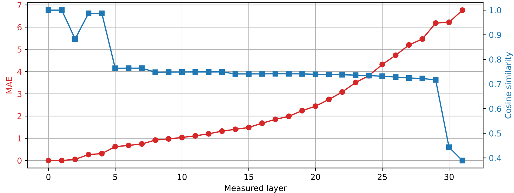
Phi-3-mini-4k-instruct | Prompt 3 Spared layer 0 | Hybrid vs unquantized
