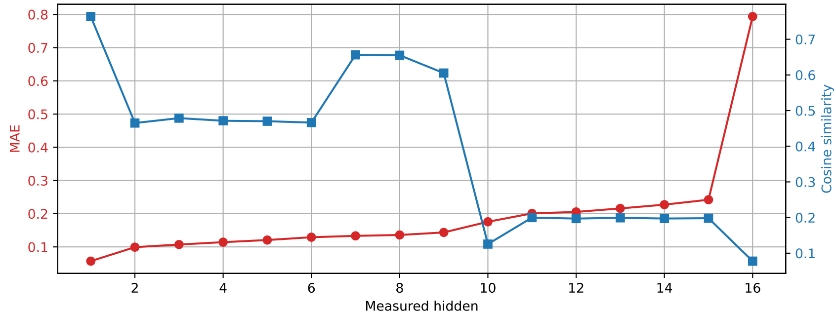
OLMo-1B-hf | Prompt 3 Spared layer 3 | Unquantized vs hybrid
