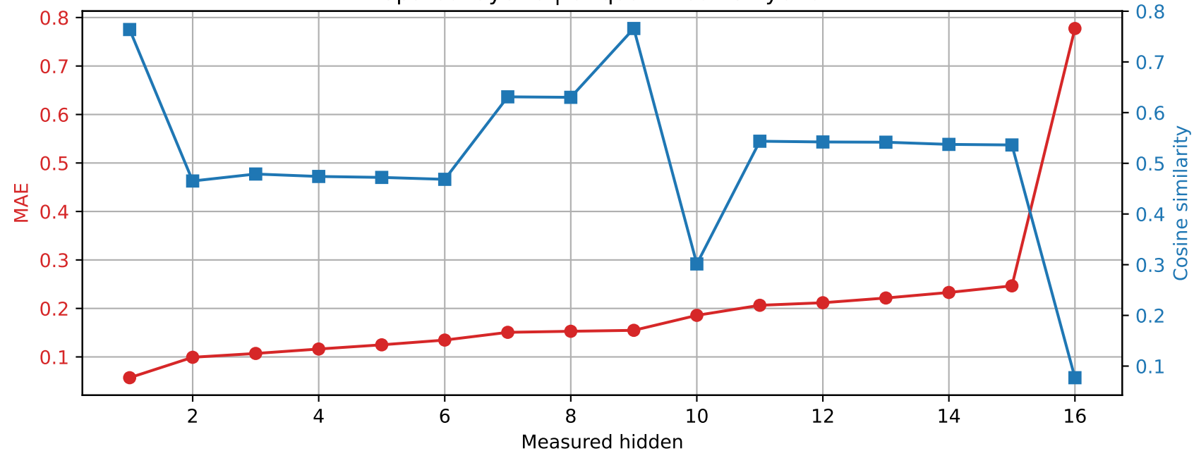
OLMo-1B-hf | Prompt 3 Spared layer 6 | Unquantized vs hybrid
