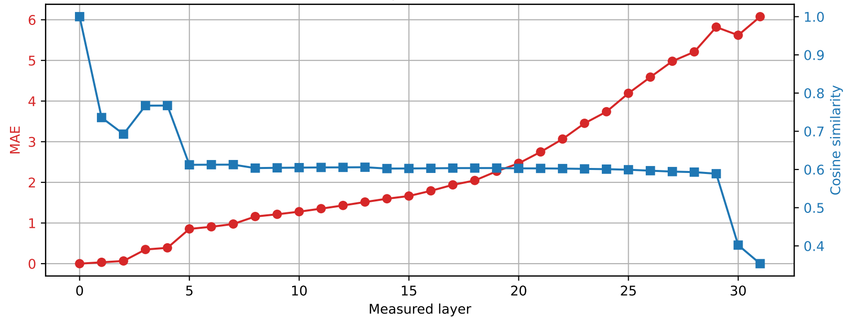
Phi-3-mini-4k-instruct | Prompt 3 Spared layer 11 | Hybrid vs unquantized
