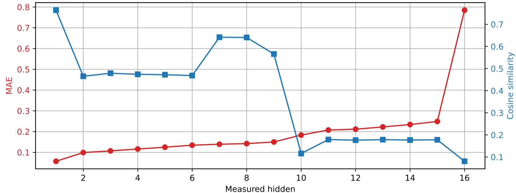
OLMo-1B-hf | Prompt 3 Spared layer 13 | Unquantized vs hybrid
