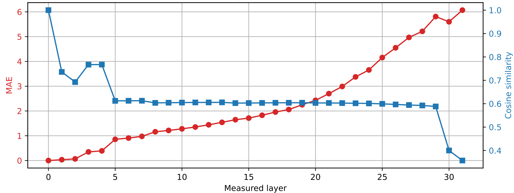
Phi-3-mini-4k-instruct | Prompt 3 Spared layer 13 | Hybrid vs unquantized
