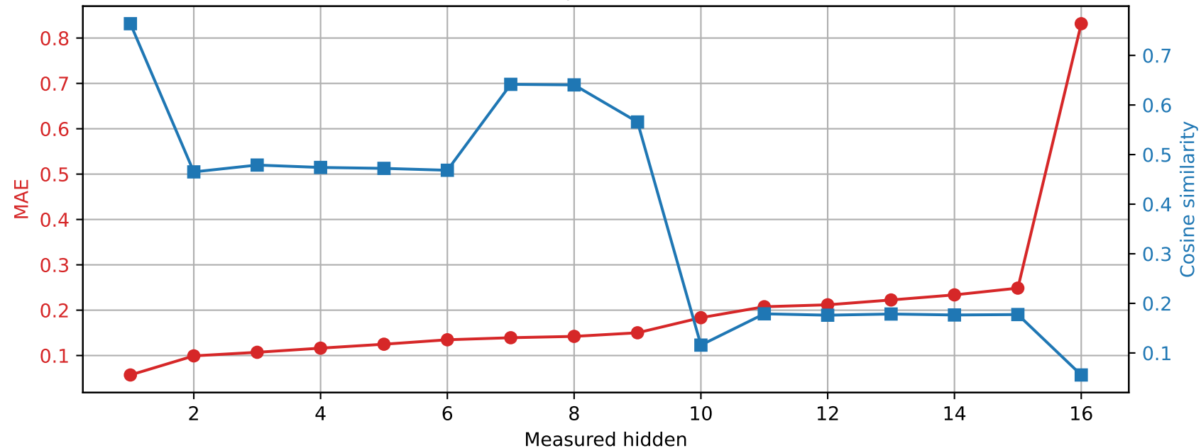
OLMo-1B-hf | Prompt 3 Spared layer 15 | Unquantized vs hybrid
