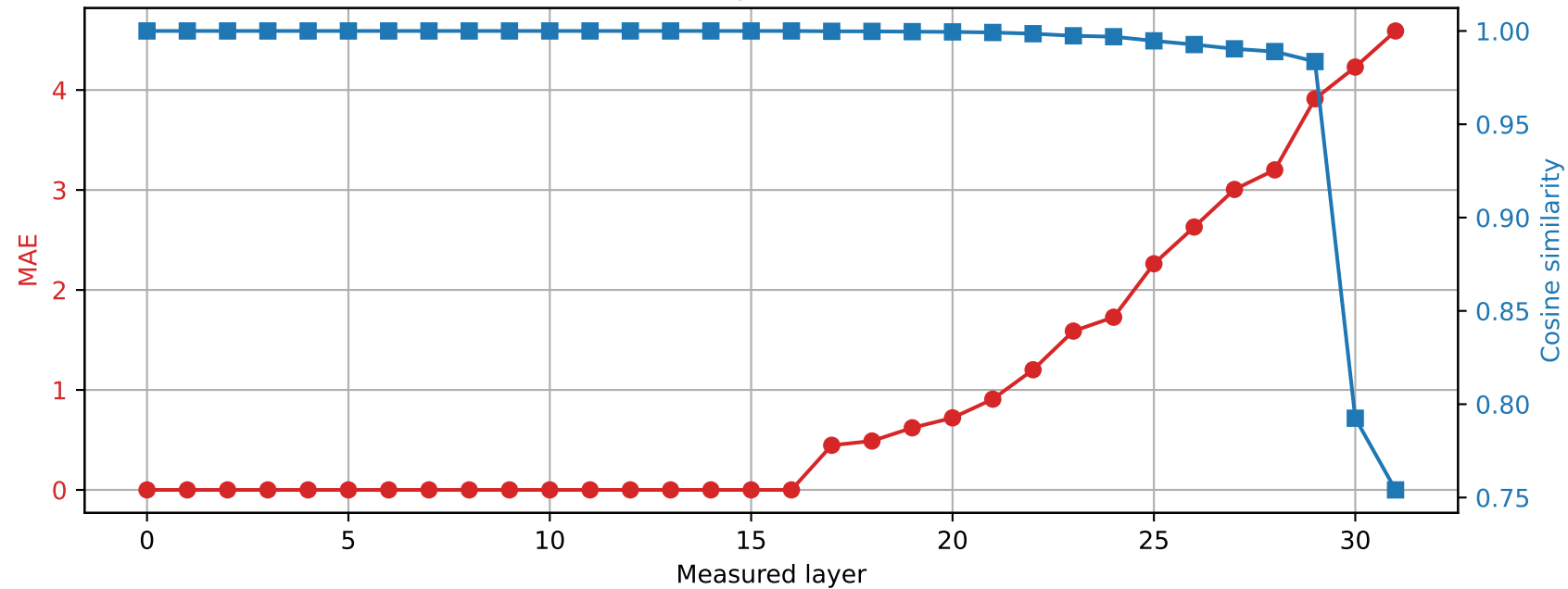
Phi-3-mini-4k-instruct | Prompt 3 Spared layer 16 | Hybrid vs quantized
