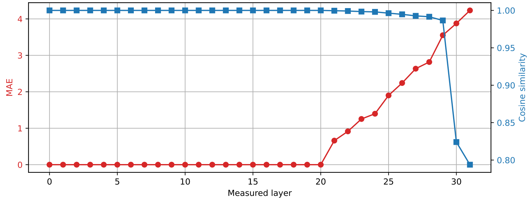
Phi-3-mini-4k-instruct | Prompt 3 Spared layer 20 | Hybrid vs quantized
