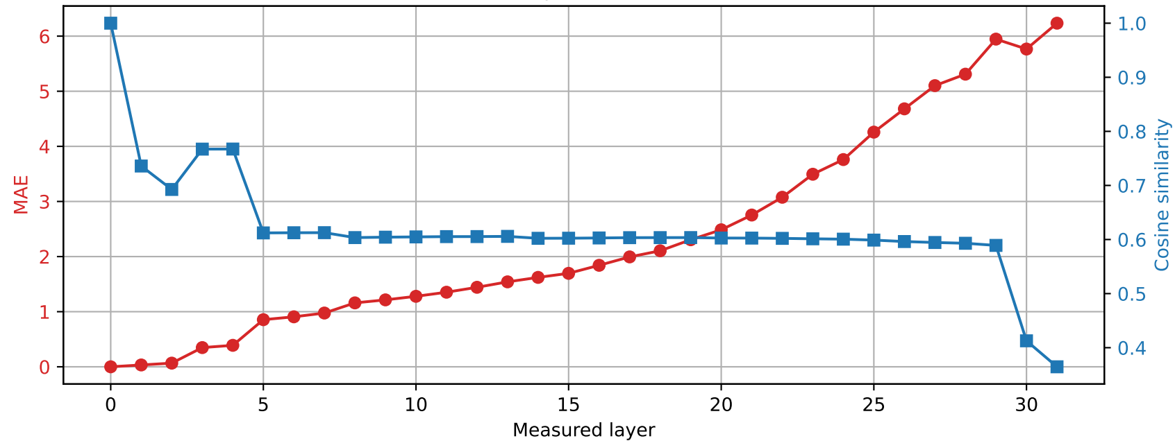
Phi-3-mini-4k-instruct | Prompt 3 Spared layer 26 | Hybrid vs unquantized
