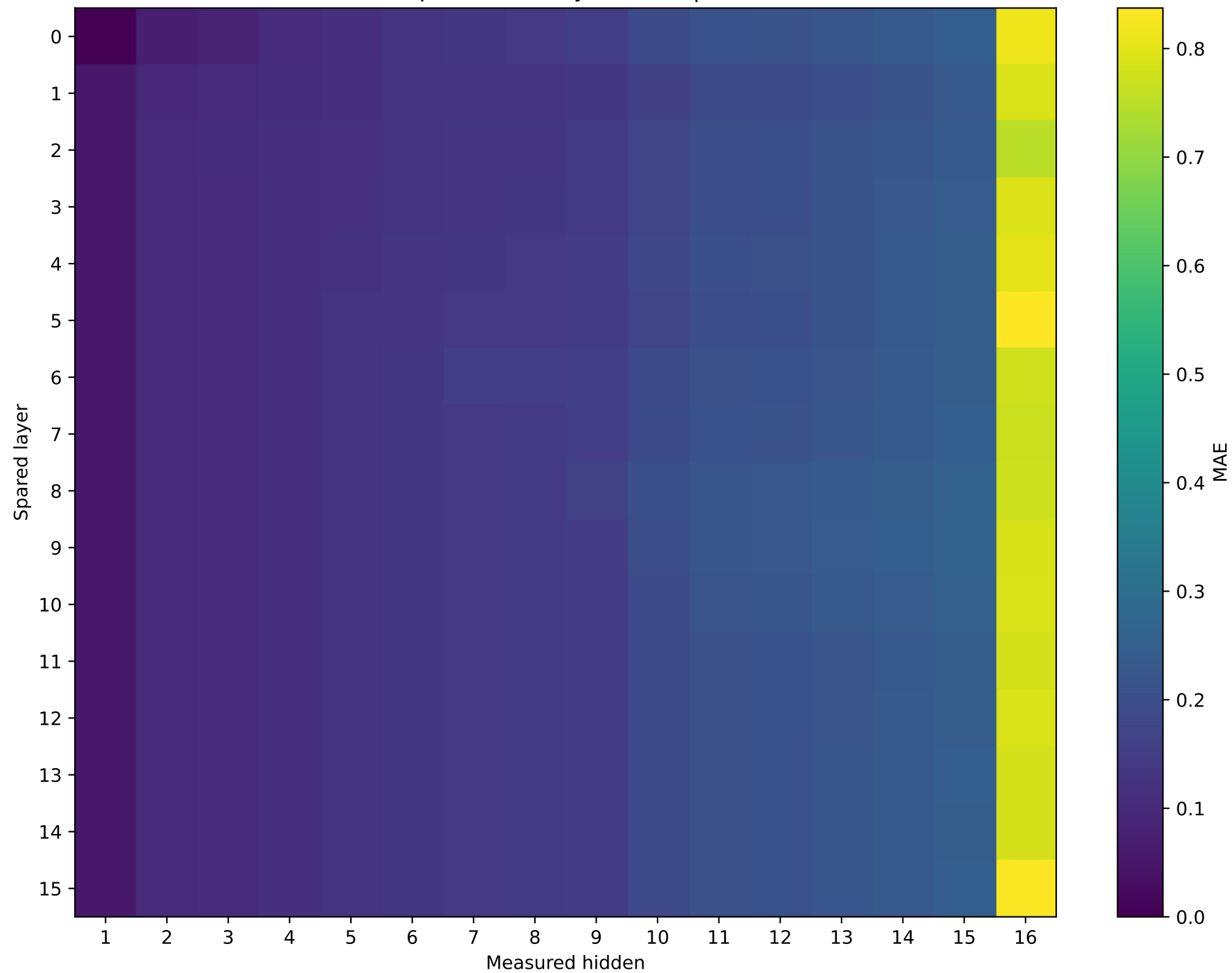
OLMo-1B-hf | Prompt 3 Unquantized vs hybrid MAE | int4
